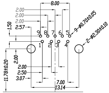
CONNECTOR FRONT EDGE REFERENCE PCB LAYOUT
