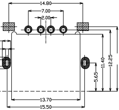
PCB LAYOUT (TOLERANCE: ±0.05) TOP VIEW (THICKNESS=1.20mm)
