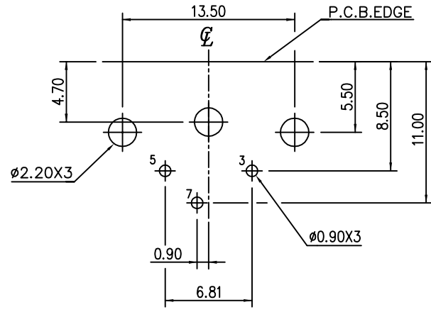
P.C.B. RECOMMEND LAYOUT (BOTTOM VIEW)
