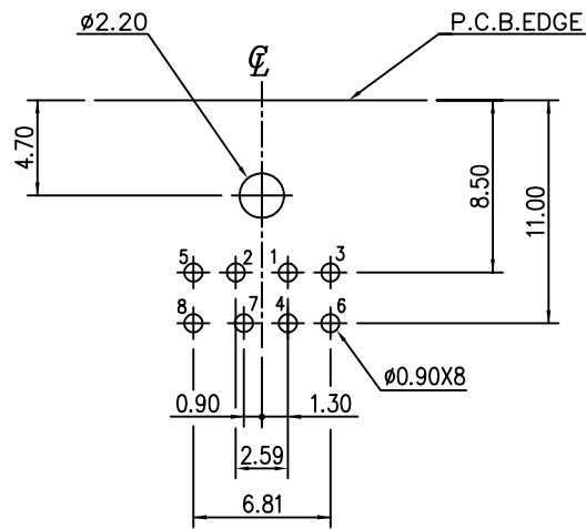
P.C.B. RECOMMEND LAYOUT (BOTTOM VIEW)
