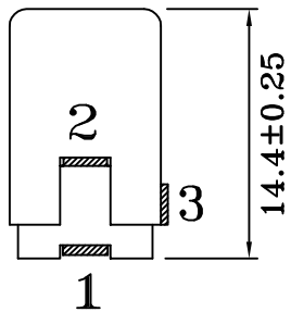
TERMINAL NUMBERS
