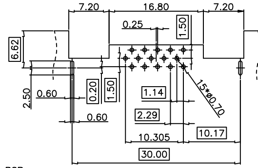
RECOMMENDED PCB LAYOUT DIMENSION TOLERANCE: ±0.05
